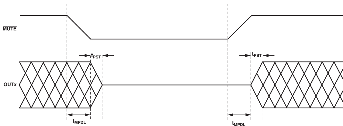
Figure 3. \overline{MUTE} Timing
