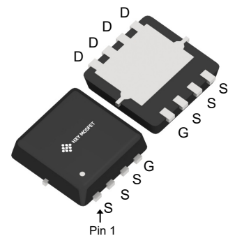
DFN3X3-8L (WDFN--8)
