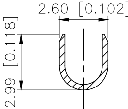
SECTION:A-A SCALE:1:1
