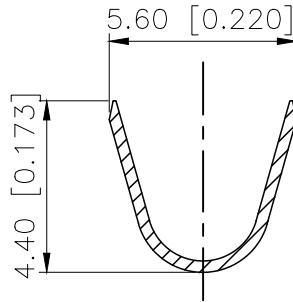
SECTION:B-B SCALE:1:1
