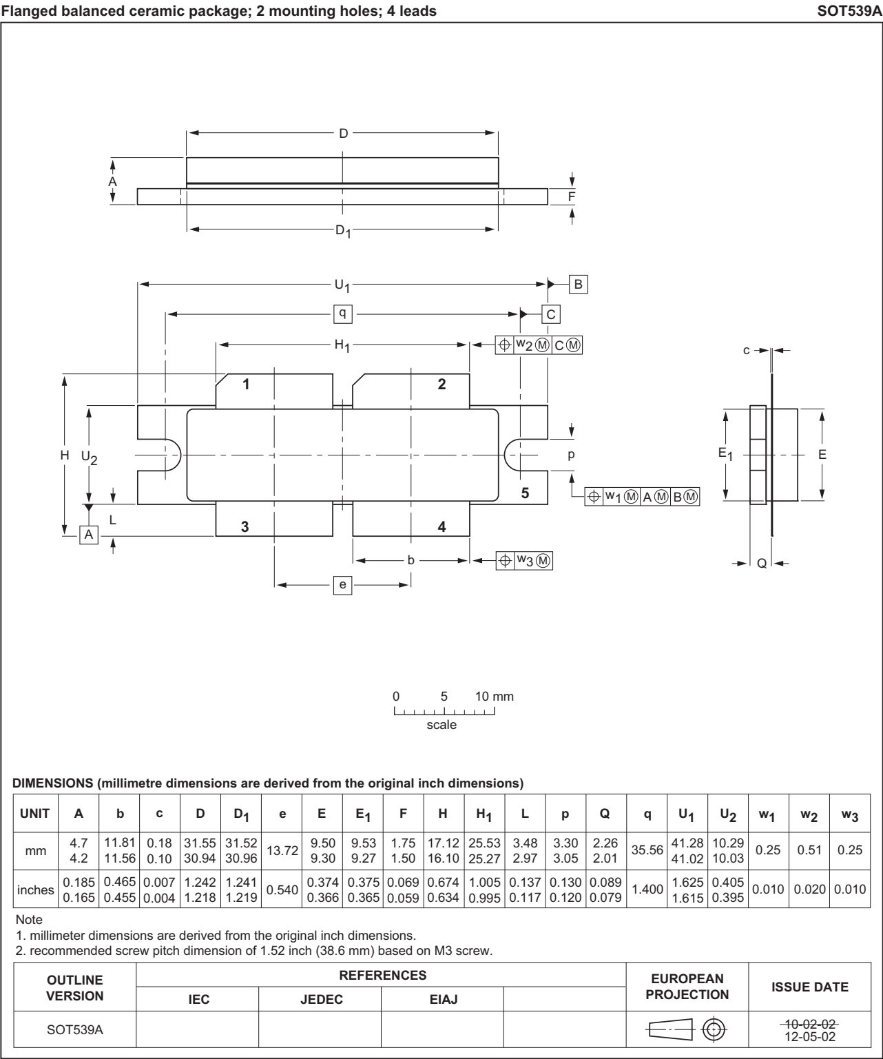
Fig 7. Package outline SOT539A
