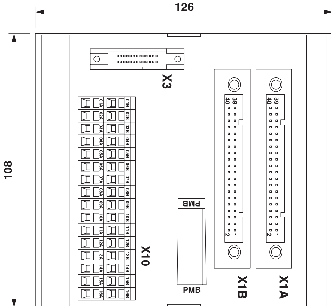
Dimensional drawing
