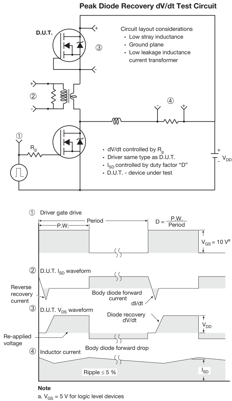
Fig. 18 - For N-Channel
