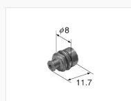
4.8mm 7165-0346
