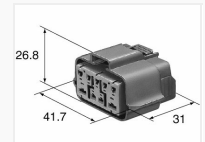
2.3/4.8mm 6195-0170
