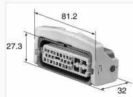
1.0/4.8mm 6189-6968
