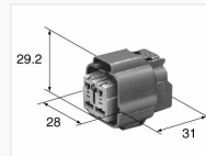
2.3/4.8mm 6195-0069
