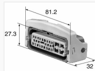
1.0/4.8mm 6189-6967
