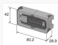
0.64/2.3/4.8mm 6189-7094
