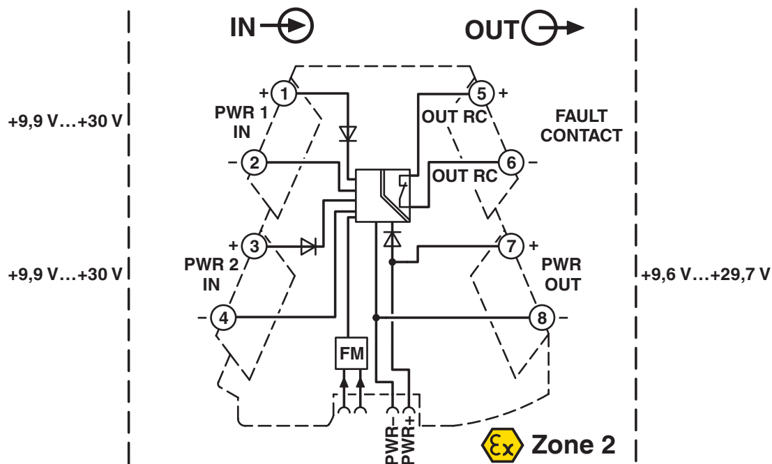
Block diagram
