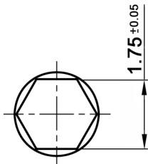
SHAFT DETAIL
