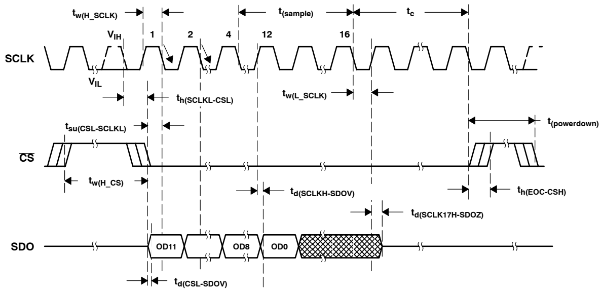
Figure 9. TLV2542 and TLV2545 Conversion Cycle Critical Timing
