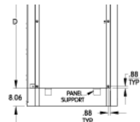
Rear View (Cross Section)
