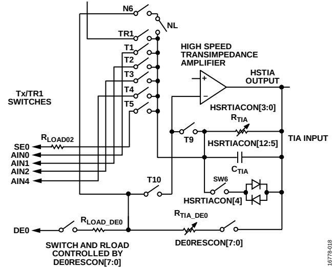
Figure 30. High Speed TIA Switches
