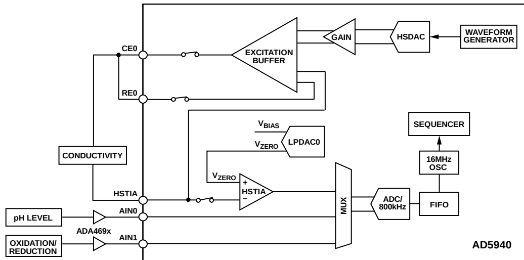
Figure 59. Typical Water Analysis Application Using the AD5940/AD5941
