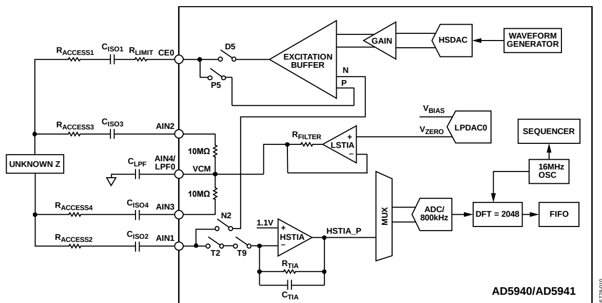
Figure 22. Low Power DACs Used in a 4-Wire Impedance Measurement (HSTIA_P = Positive Output of High Speed TIA)
