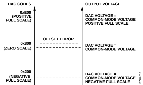
Figure 28. High Speed DAC Transfer Function
