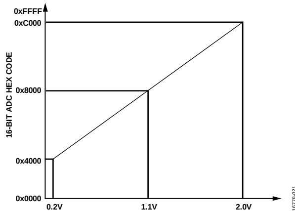
Figure 34. Ideal ADC Transfer Function, Output Codes vs. Voltage Input
