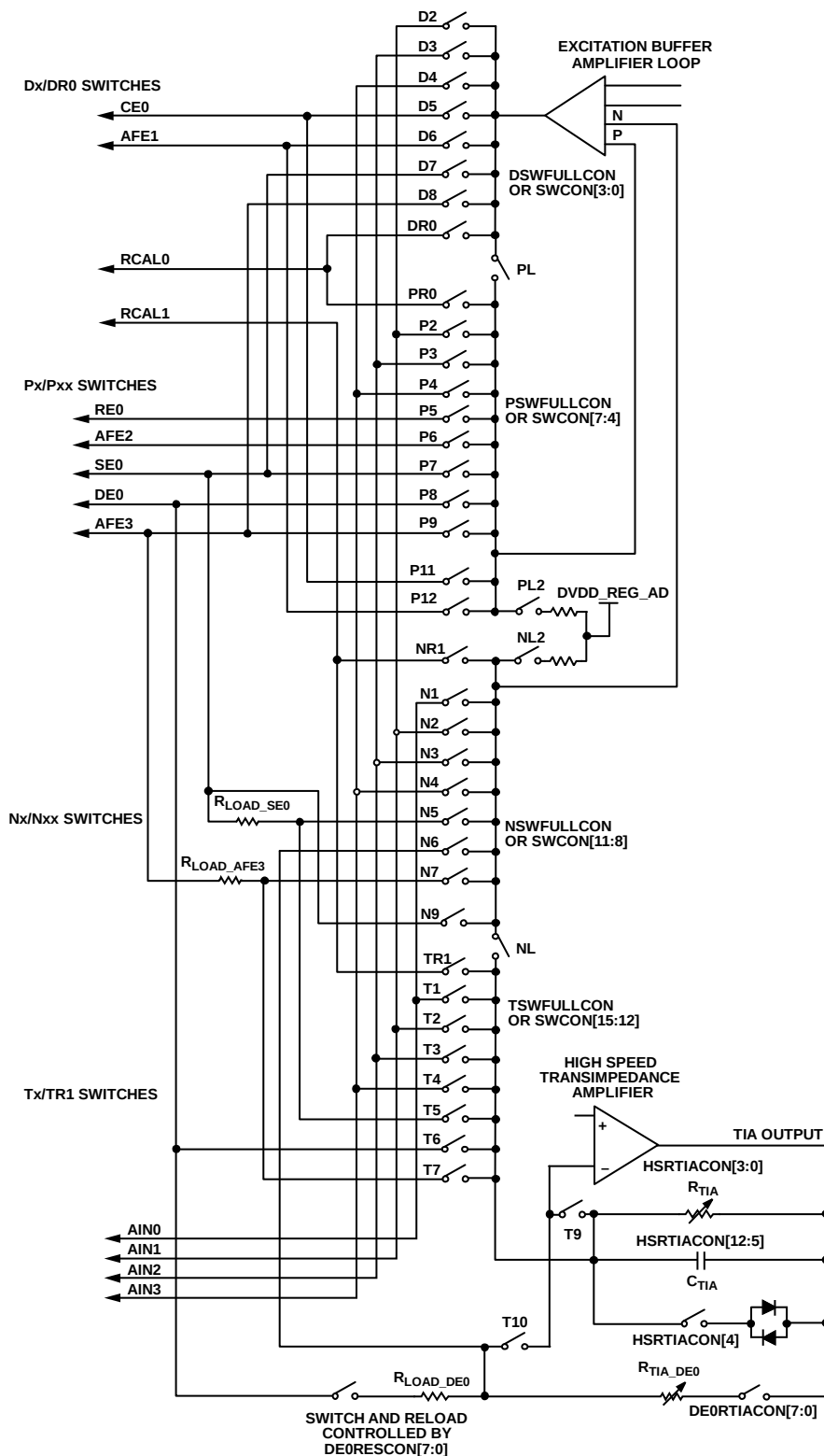
Figure 38. Switch Matrix Block Diagram—Switches Connecting to the High Speed DAC and High Speed TIA
