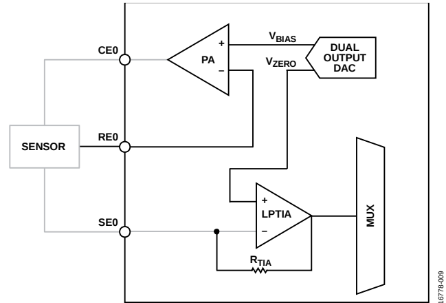
Figure 21. Electrochemical Standard Configuration
