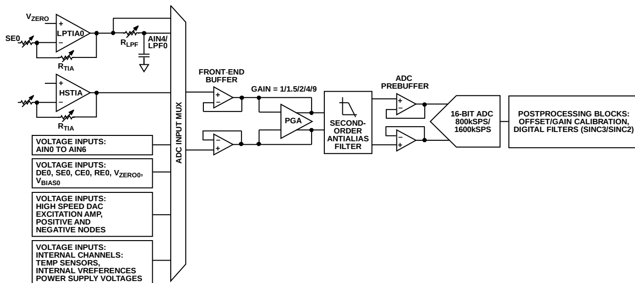
Figure 33. Basic Diagram of ADC Input Channel
