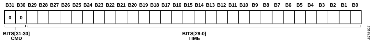
Figure 42. Sequencer Wait Command
