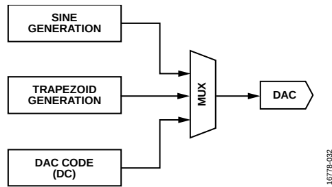
Figure 46. Simplified Waveform Generator Block Diagram
