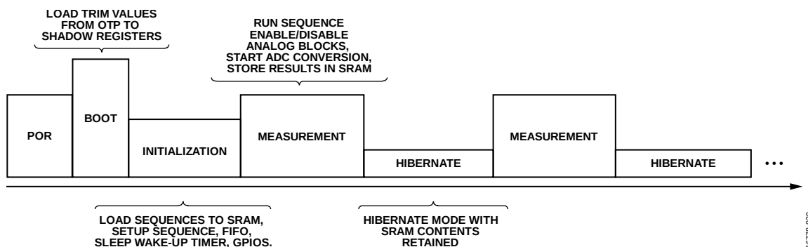
Figure 43. Run Sequence
