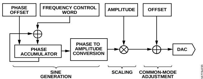
Figure 47. Sinusoid Generator
