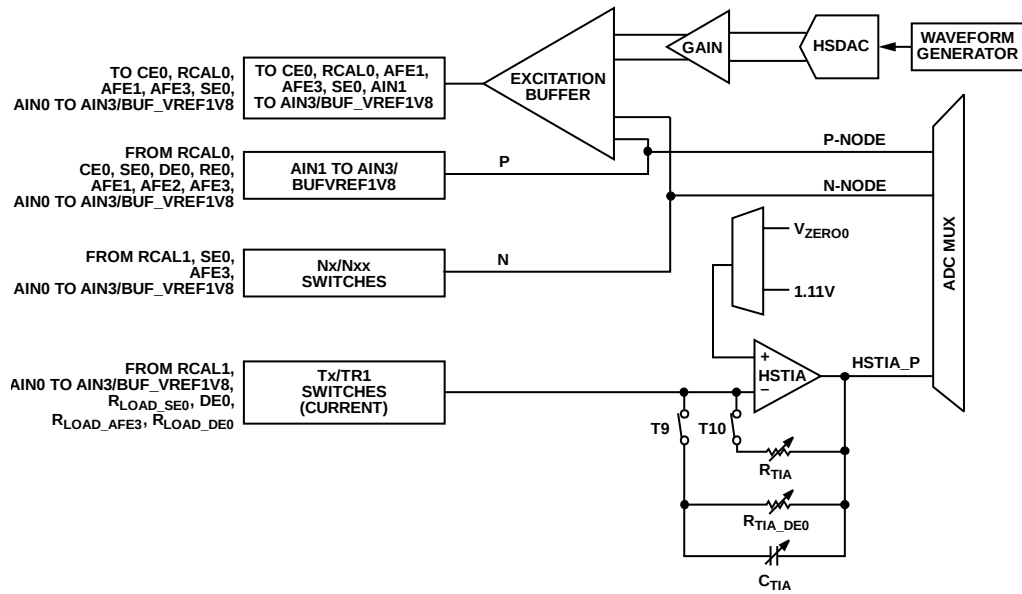
Figure 37. Switch Matrix High Level Diagram
