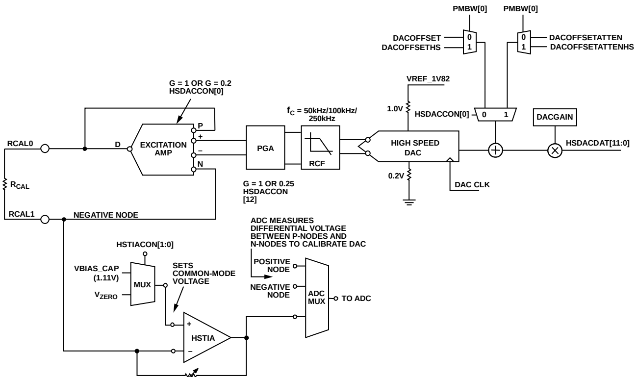
Figure 29. High Speed DAC Calibration
