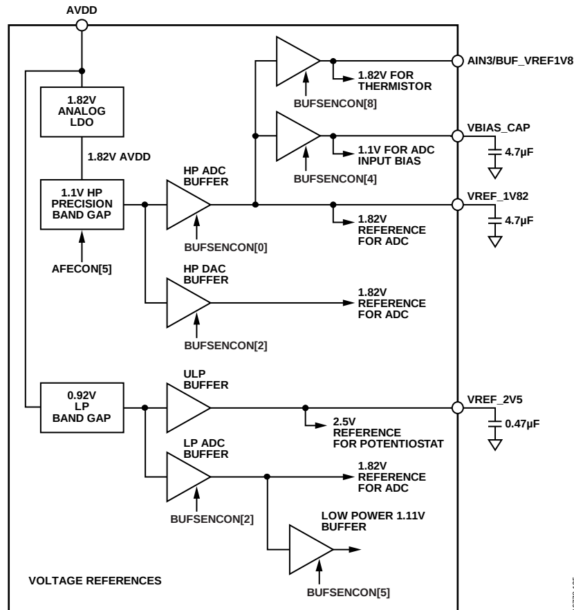
Figure 39. Precision Voltage References
