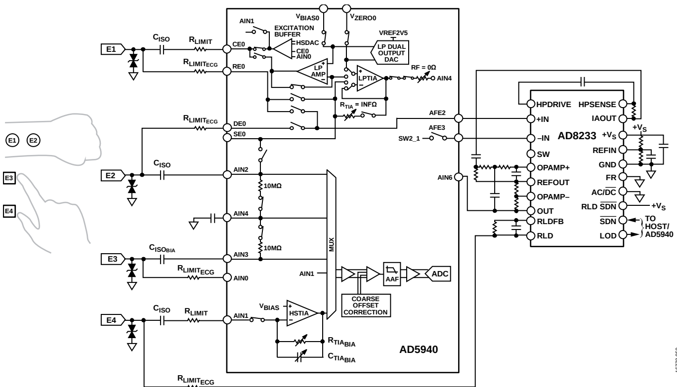
Figure 58. Body Composition and ECG System Solution Using the AD5940/AD5941 with the AD8232 and the AD8233
