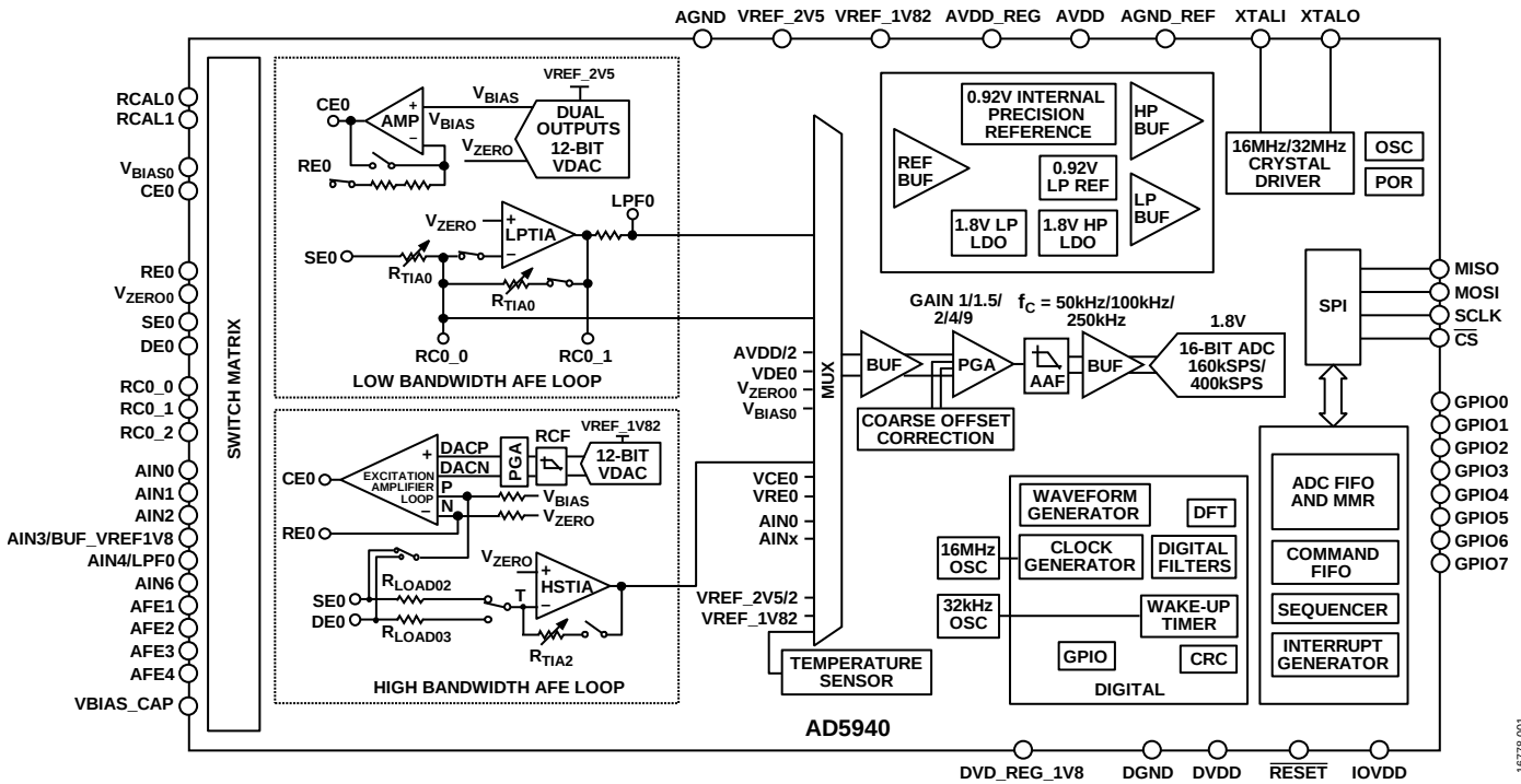
Figure 2. AD5940 Functional Block Diagram
