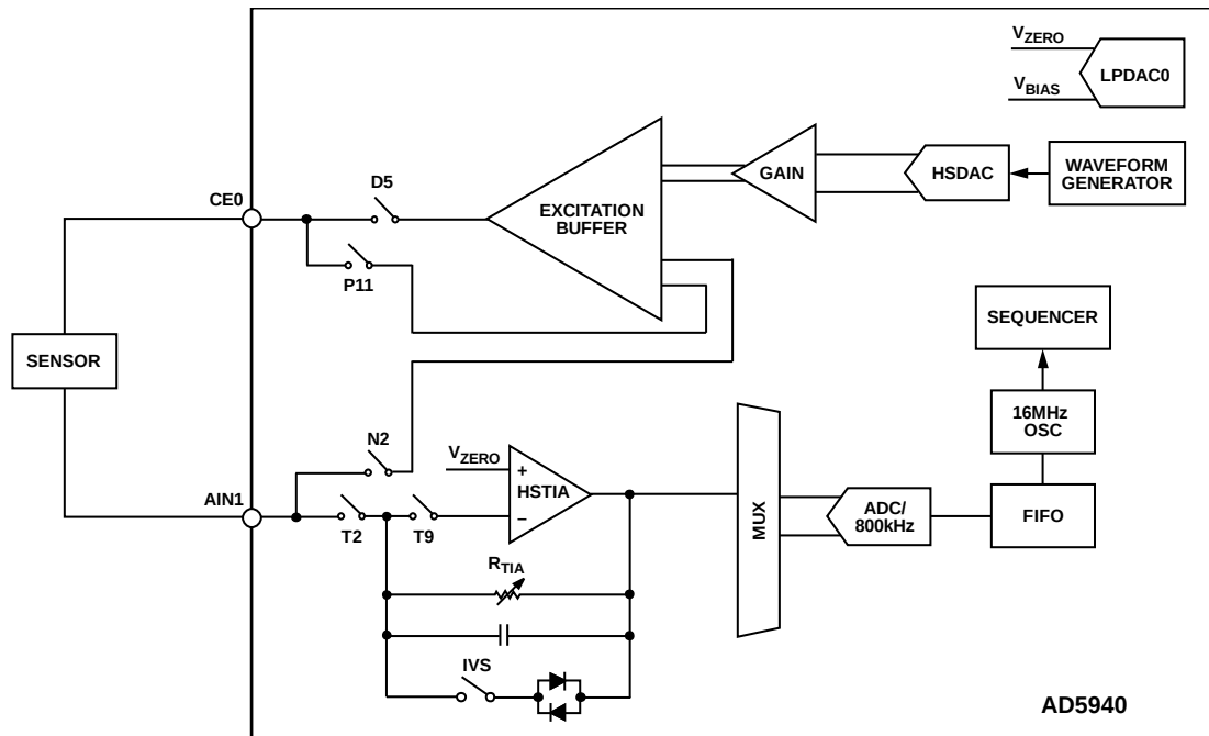
Figure 57. Using a High Bandwidth AFE Loop in Potentiostat Mode
