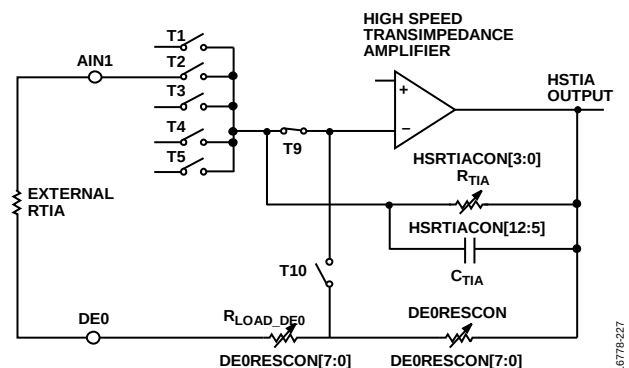
Figure 31. Connecting External R_{\text{TIA}} to the High Speed TIA
