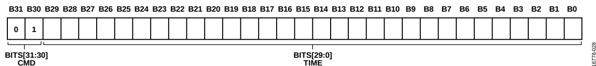
Figure 41. Sequencer Timer Command
