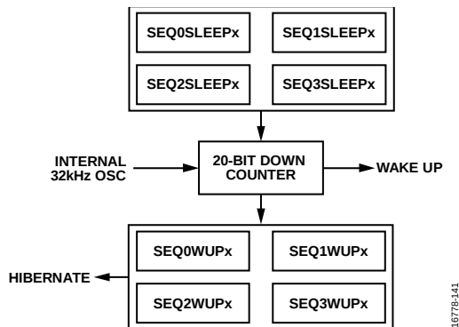
Figure 50. Sleep and Wake-Up Timer Block Diagram
