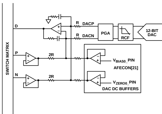
Figure 26. High Speed DAC Excitation Amplifier
