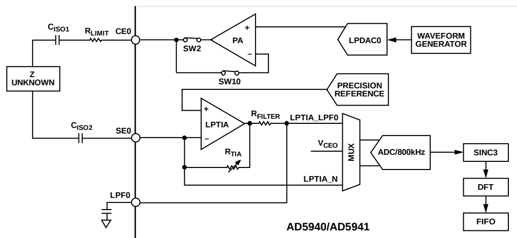
Figure 55. Low Frequency, 2-Wire, Bioimpedance Loop (Maximum Bandwidth = 300 Hz)
