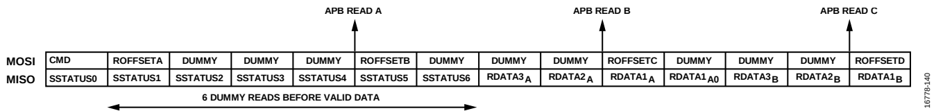
Figure 49. Data FIFO Read Protocol
