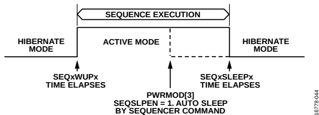
Figure 51. Sleep and Wake-Up Timing Diagram
