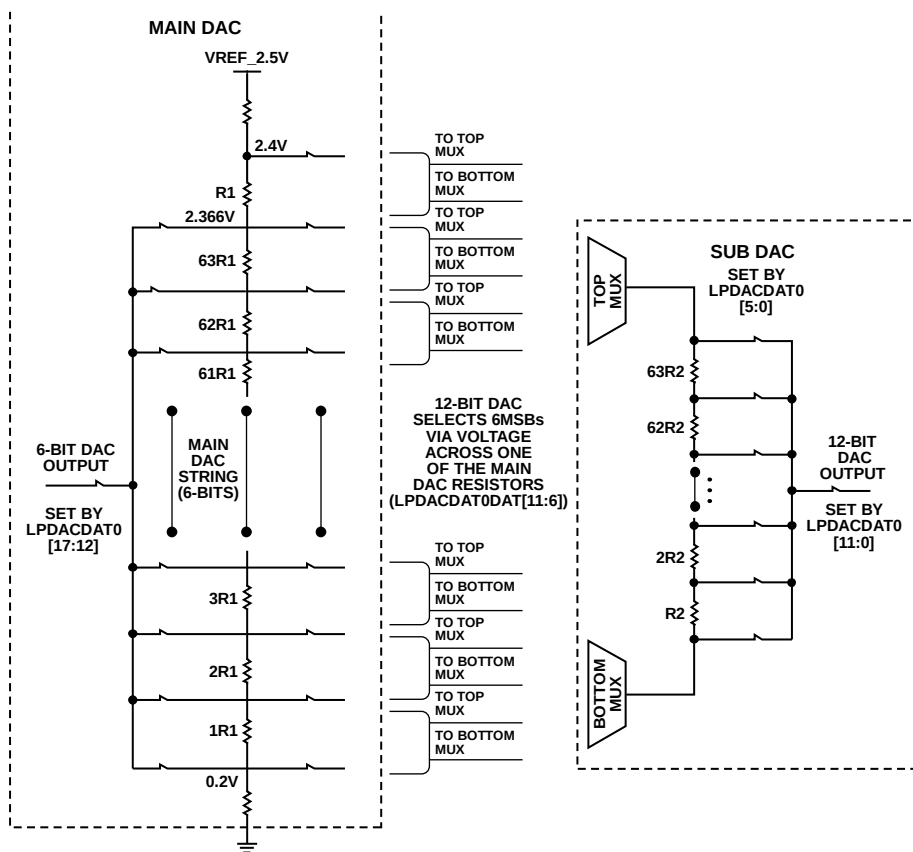
Figure 20. Low Power DAC Resistor String
