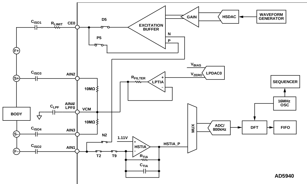
Figure 56. High Frequency, 4-Wire, Bioimpedance Loop (Maximum Bandwidth = 200 kHz)
