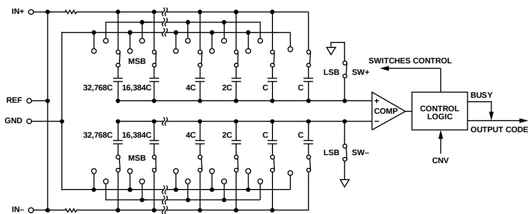
Figure 32. ADC Core Block Diagram (IN+, REF, GND, and IN- are Internal Nodes)
