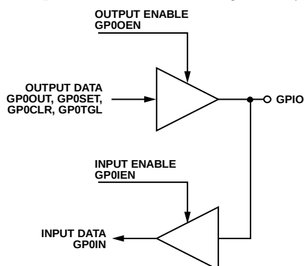
Figure 53. Digital Input/Output Diagram
