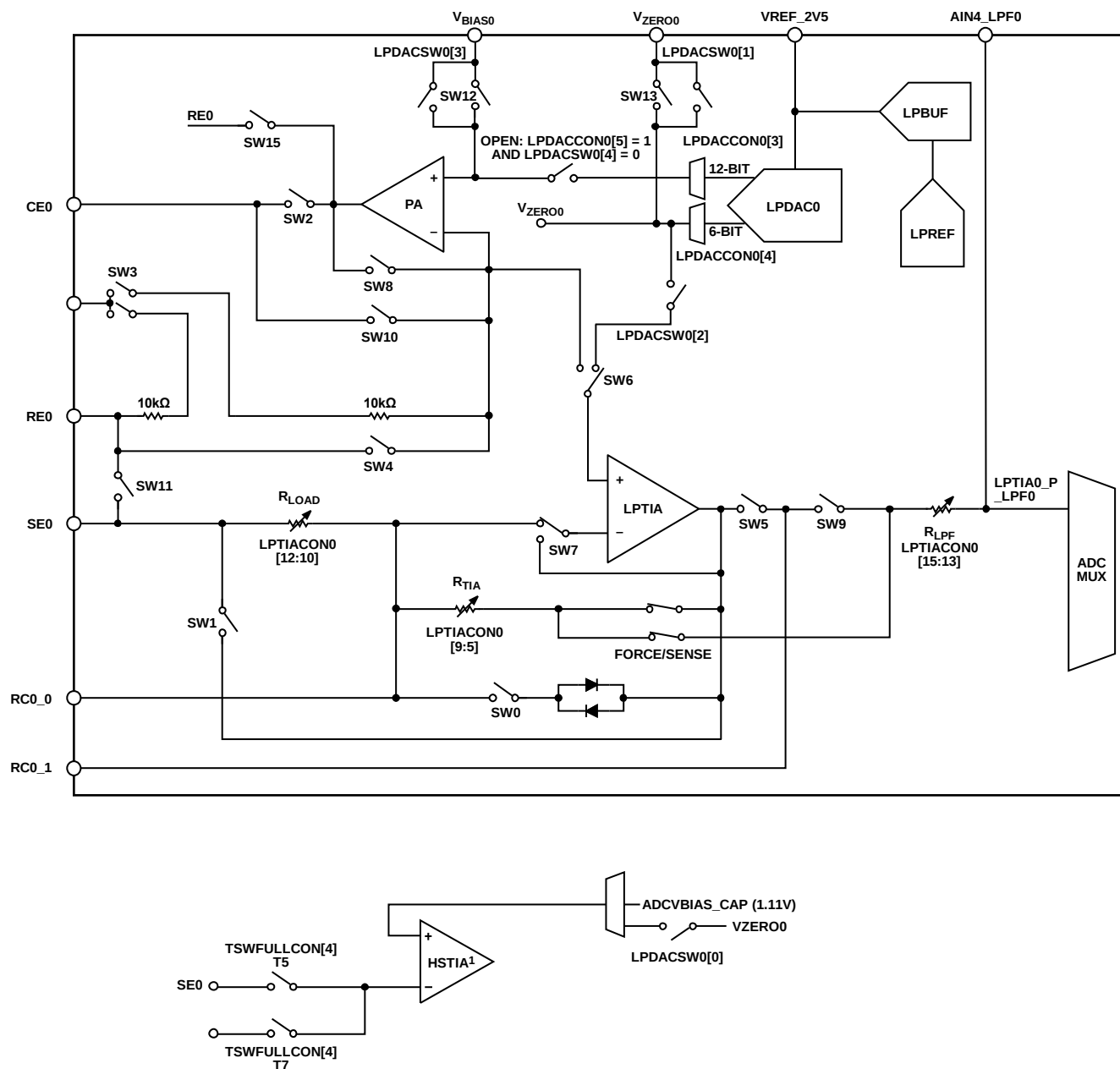
Figure 24. Low Bandwidth Loop Switches
