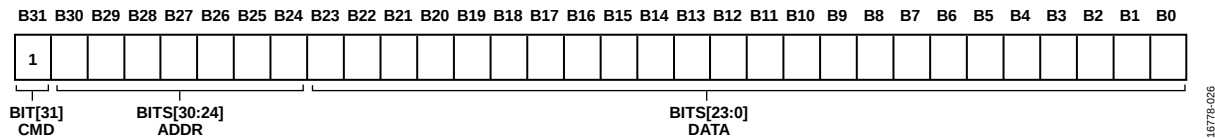
Figure 40. Sequencer Write Command
