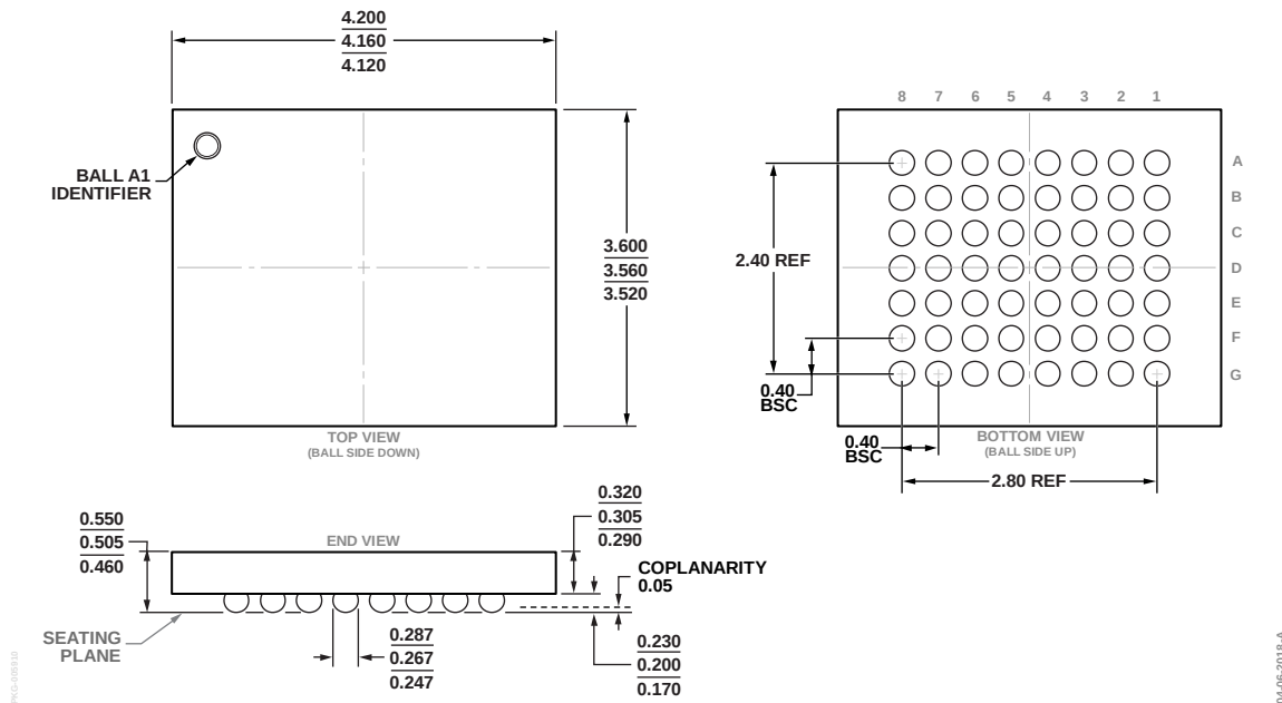
Figure 60. 56-Ball Wafer Level Chip Scale Package [WLCSP] (CB-56-3)
