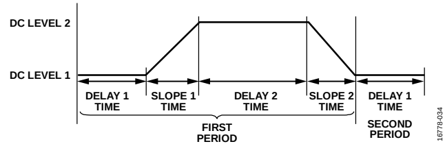
Figure 48. Trapezoid Waveform Definition
