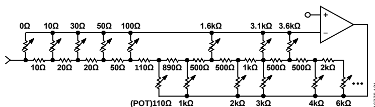
Figure 23. LPTIA R_{LOAD} and R_{GAIN} Configuration
