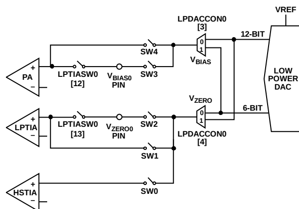
Figure 19. Low Power DAC Switches
