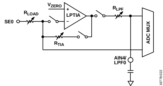
Figure 35. Low Power TIA Current Input Channel to the ADC
