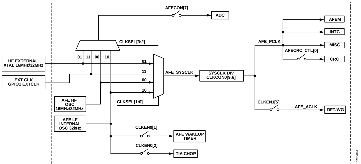
Figure 54. AD5940/AD5941 System Clock Architecture
