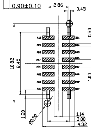
RECOMMENDED P.C.B. LAYOUT (俯视图) TOLERANCE UNSPECIFIED ±0.05mm
