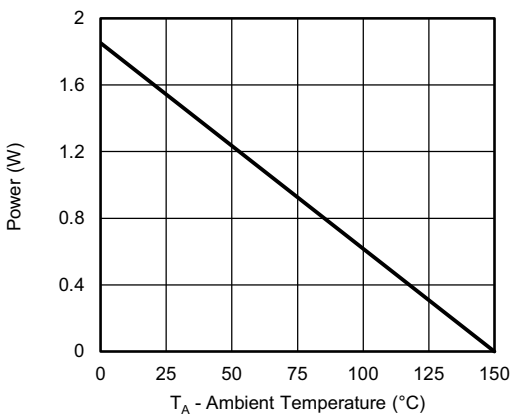
Power, Junction-to-Ambient
