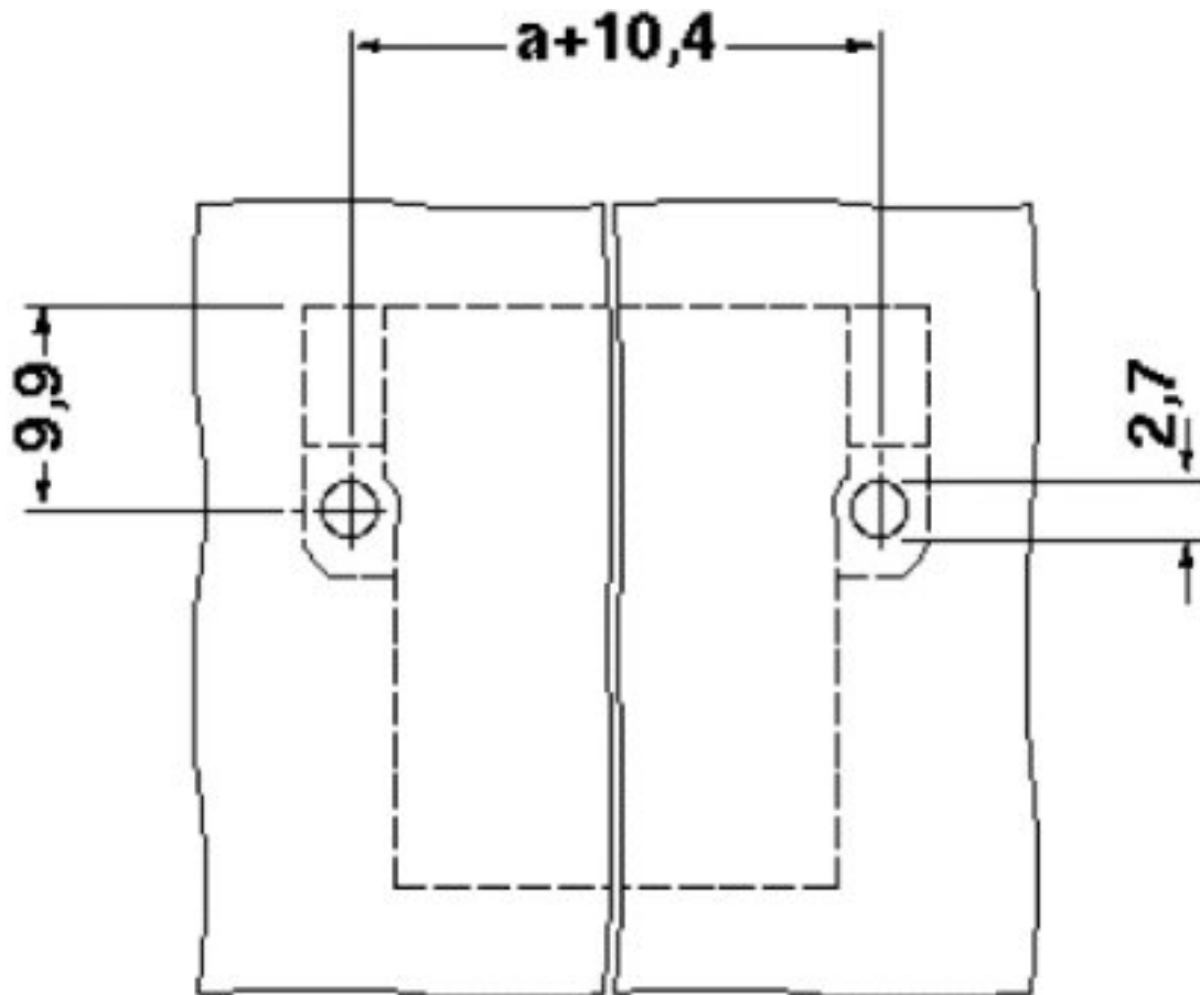
Dimensional drawing
