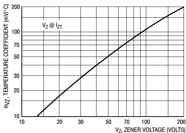
Figure 4. Zener Voltage – 14 To 200 Volts
