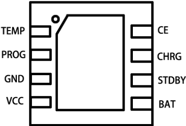
DFN2X2-8L
