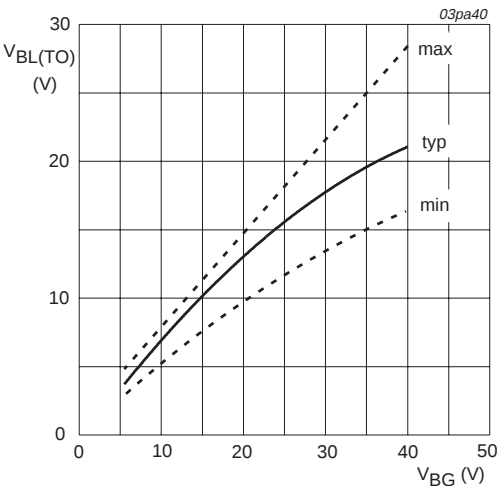
Fig 11. Battery-load threshold voltage as a function of battery-ground voltage.
