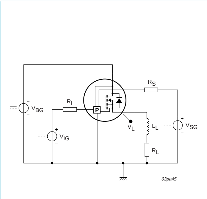
Fig 12. Schematic drawing of the switching circuit.
