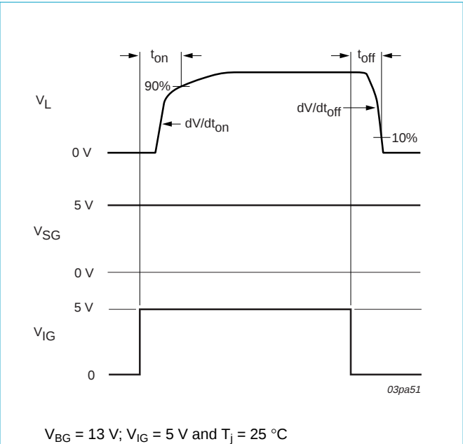
Fig 13. Resistive switching waveforms and definitions.
