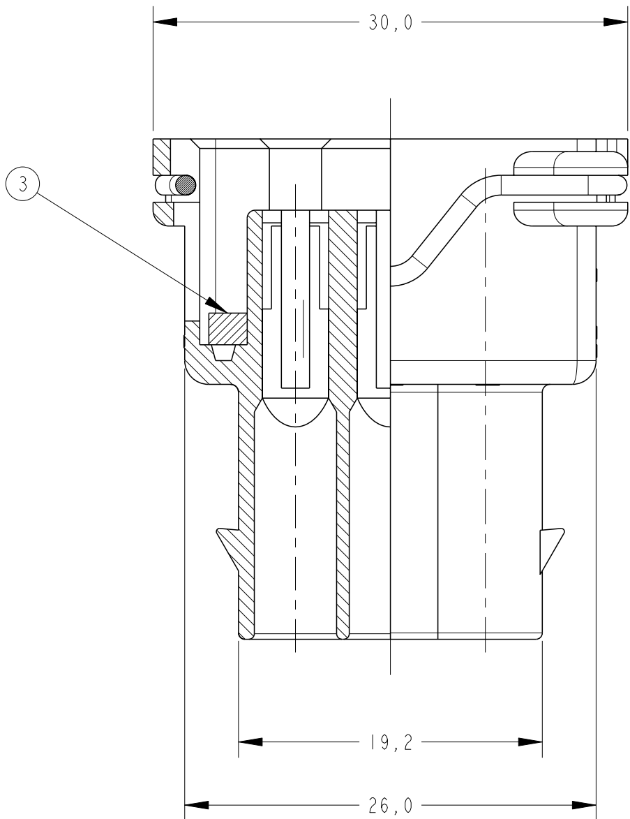
SECTION B-B
