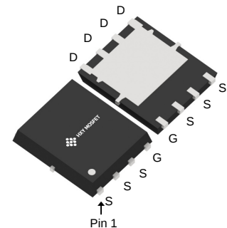
DFN5X6-8L (DFN-5(5.1x6.1))
