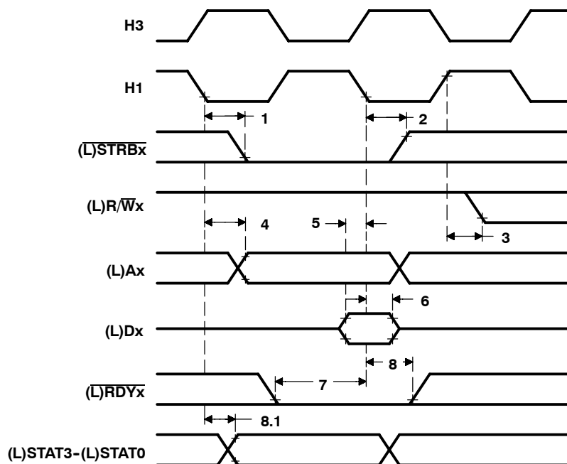
Figure 10. Memory-Read-Cycle Timing [ (\overline{\text{L}})\text{STRBx} = 0 ]
