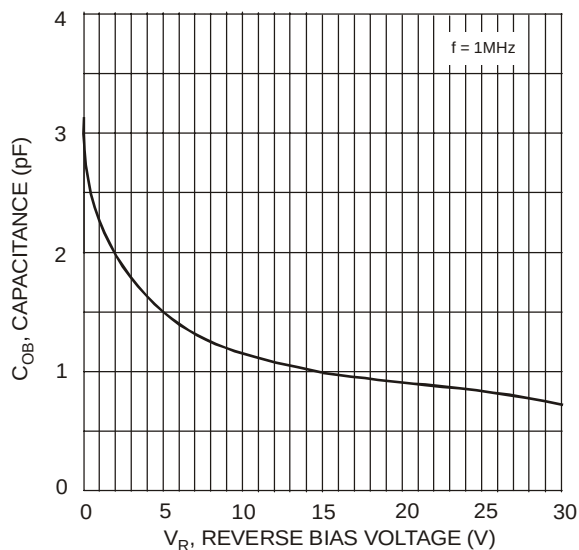
Fig. 4 Output Capacitance
