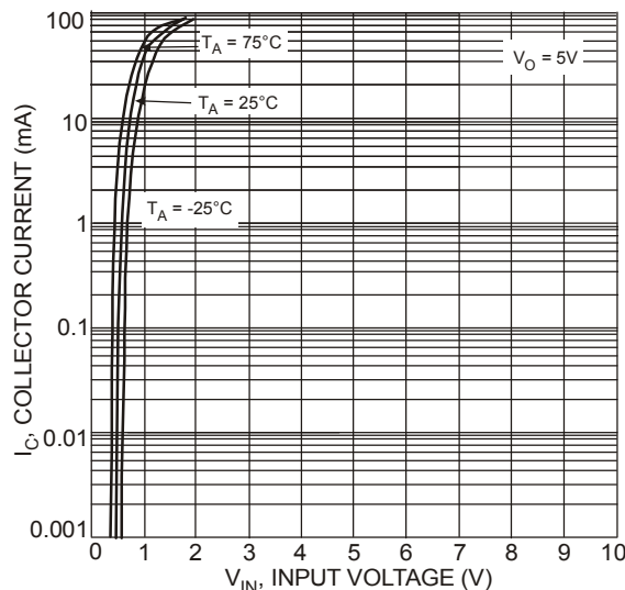
Fig. 10 Typical Collector Current vs. Input Voltage
