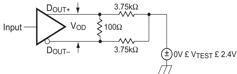
Figure 2. V_{OD} Test Circuit
