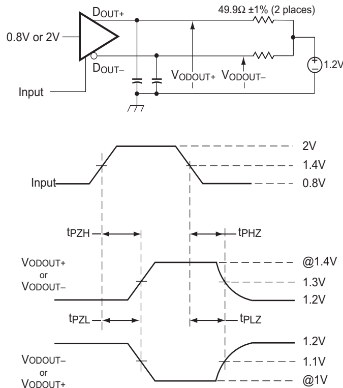
Figure 4. Test Circuit, Timing, & Voltage Definitions for the Differential Output Signal
