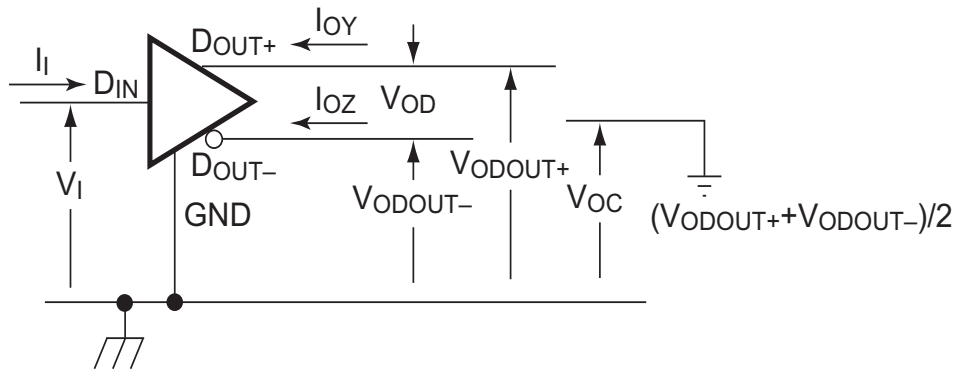
Figure 1. Voltage and Current Definitions
