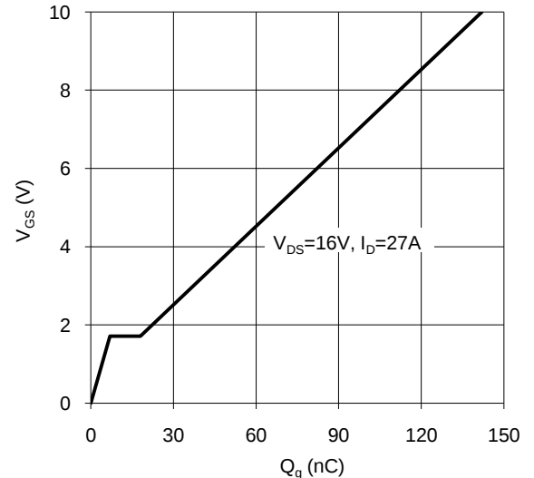
Figure 12. Gate Charge
