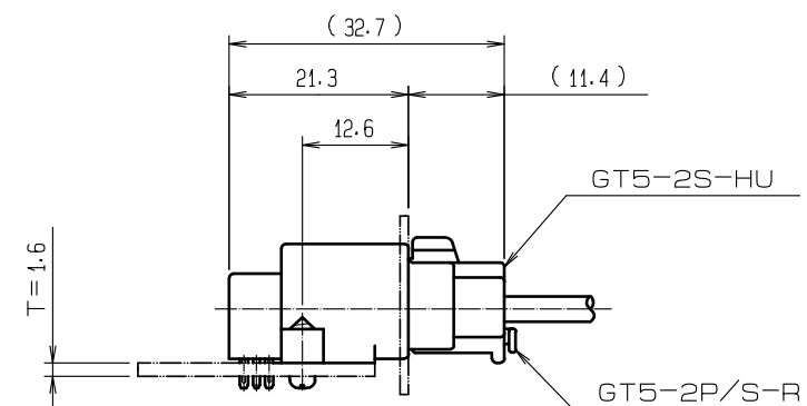
MATED CONNECTORS
