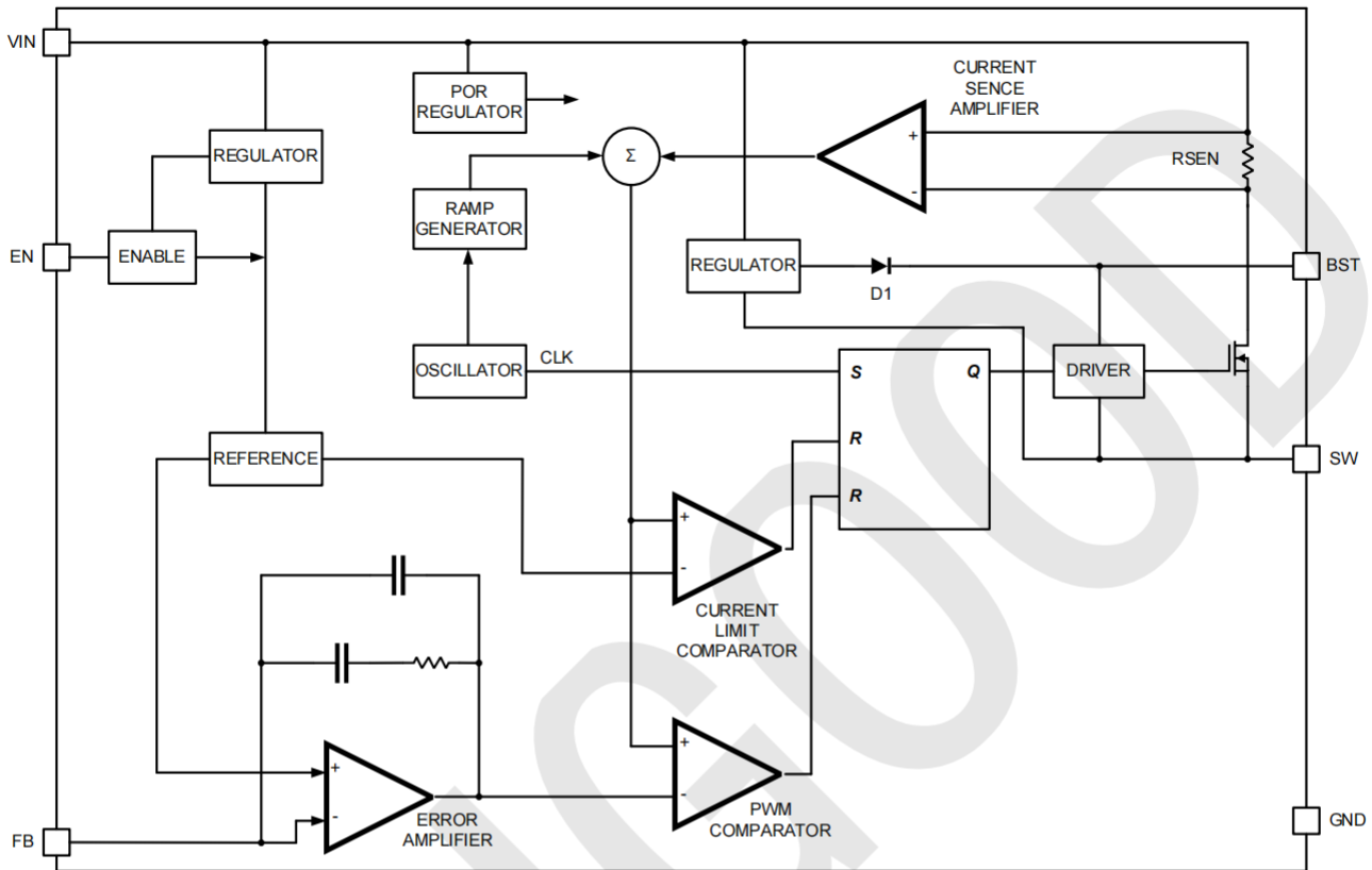
Block Diagram
