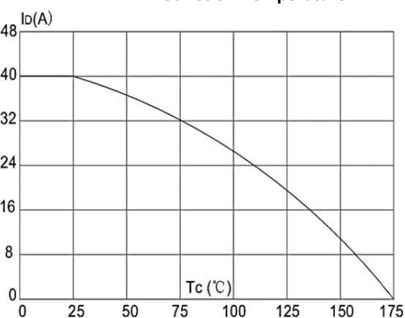
Figure 10: Maximum Continuous Drain Current vs. Ambient
