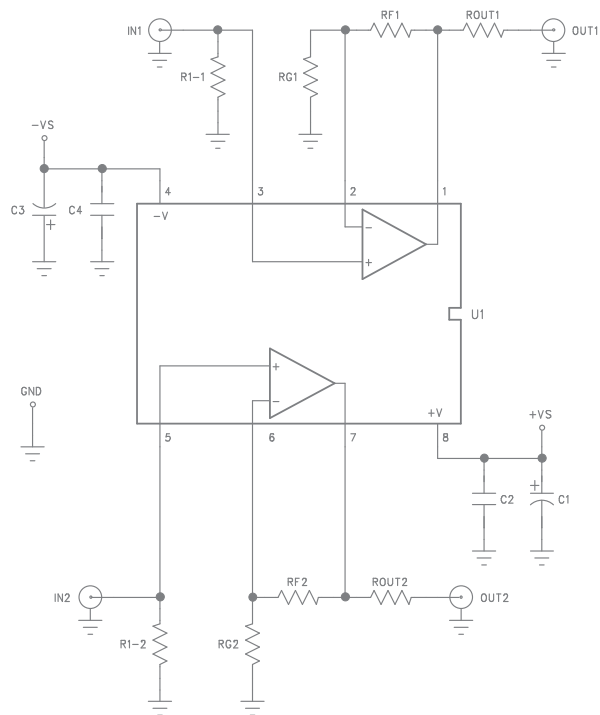
Figure 12. CEB006 Schematic
