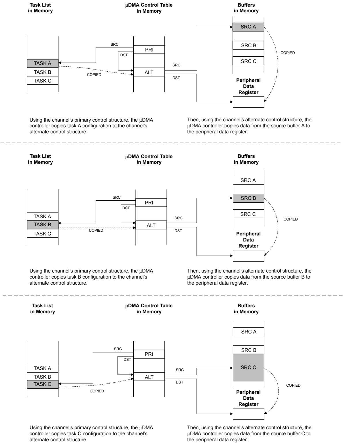
Figure 7-6. Peripheral Scatter-Gather, μDMA Copy Sequence
