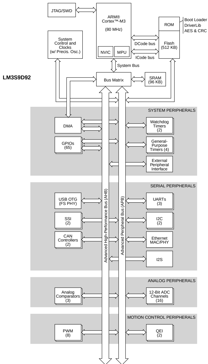
Figure 1-1. Stellaris LM3S9D92 Microcontroller High-Level Block Diagram
