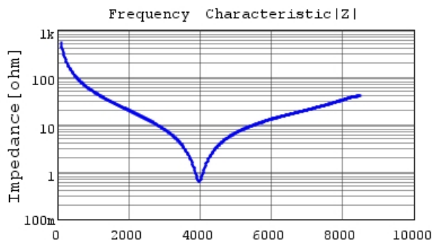
GRM1885C1H3R0WA01 |Z| DCOV, 25degC
