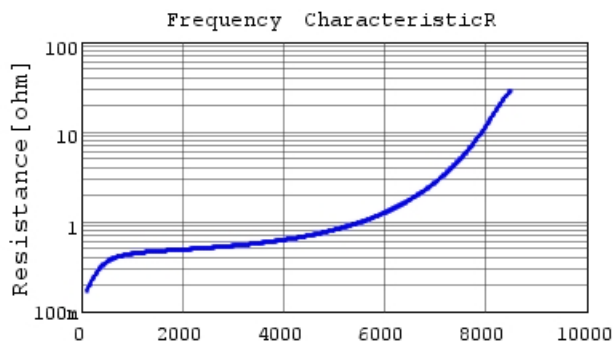
GRM1885C1H3R0WA01 R DCOV, 25degC
