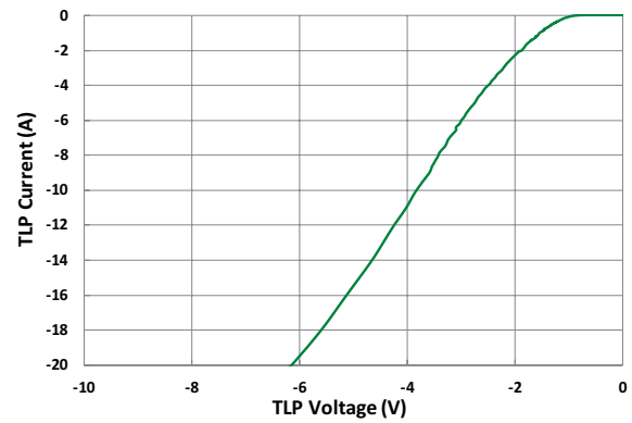
Negative Transmission Line Pulsing (TLP) Plot
