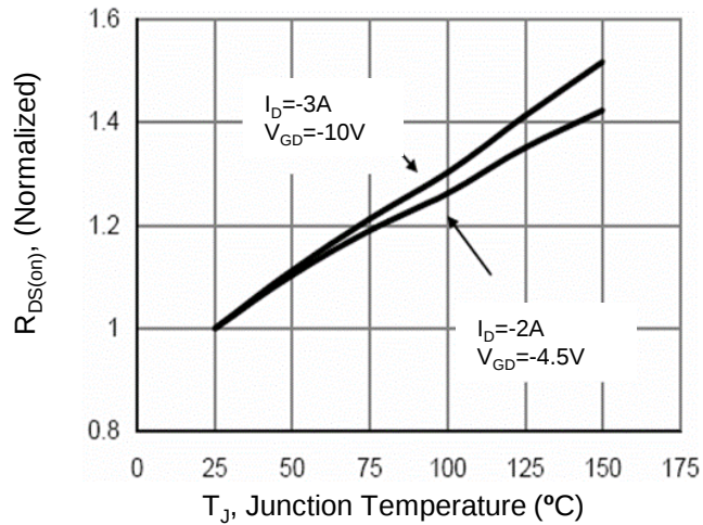
Figure 7. Drain-Source On-Resistance
