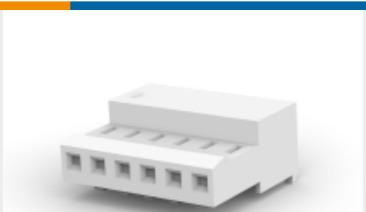
TE Part #3-641535-6 06P MTA100 CONN ASSY 24AWG
