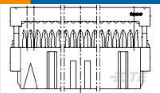
TE Part #6-215882-4 64 WAY GREY MK II RECP
