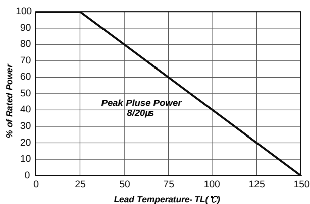
Fig2.Power Derating
