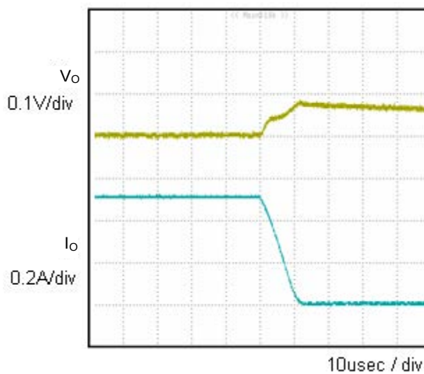
Fig.4 Transient Response (0.5→0A) C_o=1\mu\text{F}
