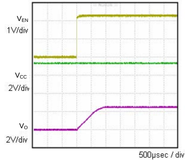
Fig.7 Input sequence 2 Co=1μF
