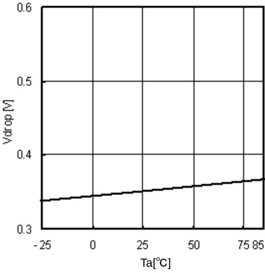
Fig.18 Minimum dropout Voltage 1 ( V_{CC}=3.3V , I_O=-0.5A )
