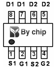
Pin Assignment
