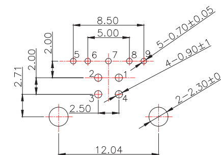
REFERENCE PCB LAYOUT
