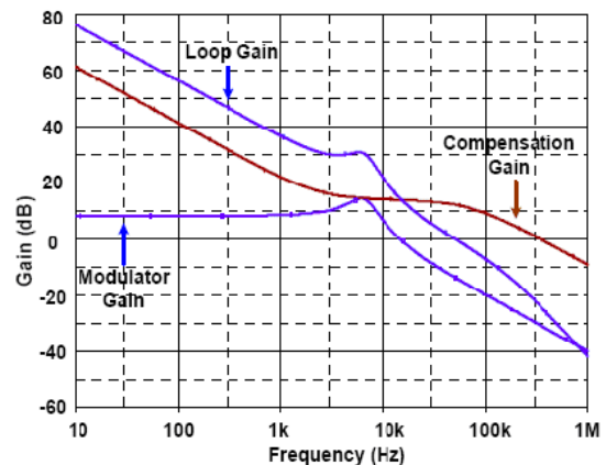
Figure 25. Bode Plot
