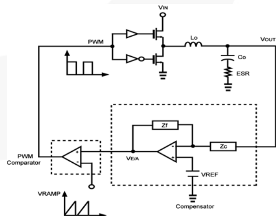
Figure 23. Closed Loop
