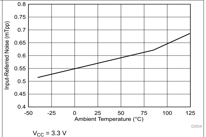
Figure 6. DRV5053AD, B_N vs Temperature
