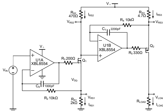
Figure 8. Bidirectional Current-Sensing
