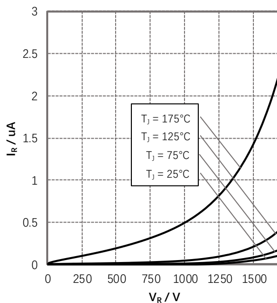
Figure 2. Reverse Characteristics
