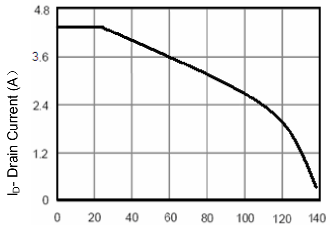
T_J -Junction Temperature( ^\circ\text{C} ) Figure 2 Drain Current
