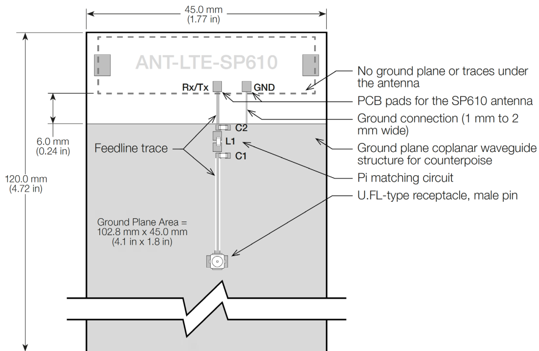
Figure 9. SP610 Recommended Layout.
