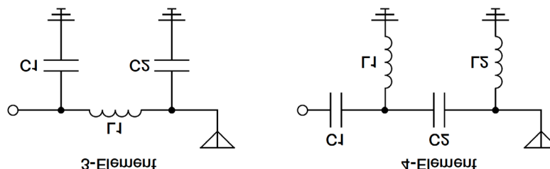
Figure 10. Matching Network Recommendations
