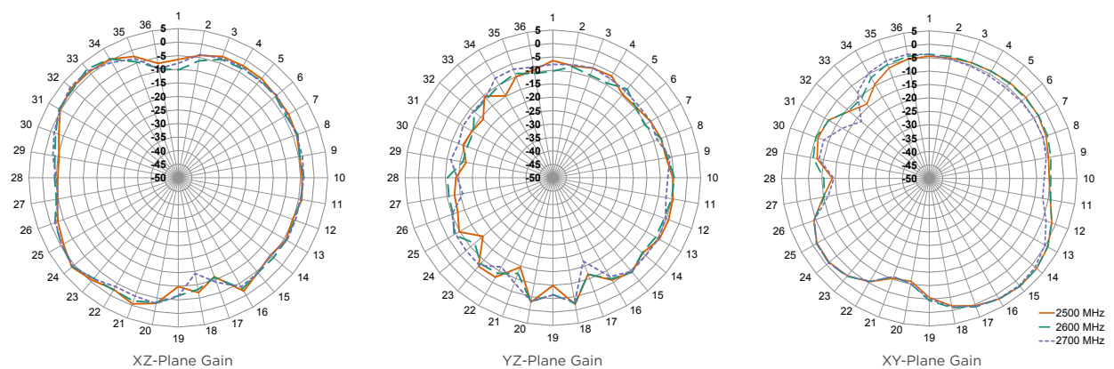
Figure 8. Radiation Patterns for the SP610 Antenna
