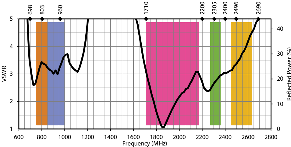
Figure 1. SP610 VSWR with Frequency Band Highlights
