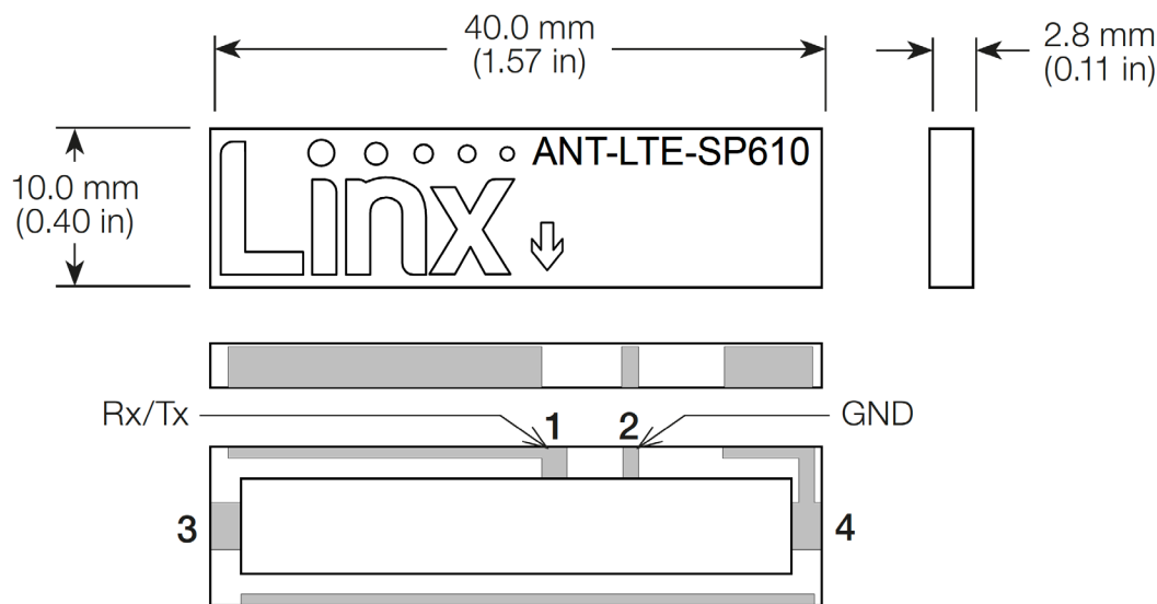
Figure 6. SP610 Dimensions
