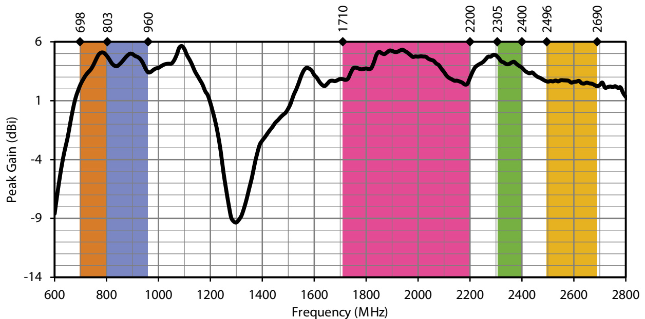
Figure 3. SP610 Peak Gain with Frequency Band Highlights
