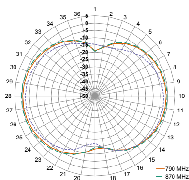
XY-Plane Gain
