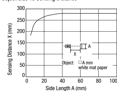
Object Size vs Sensing Distance
