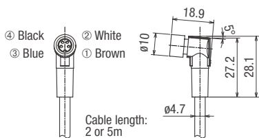
Right-angle (SA9Z-CM8K-4L□)
