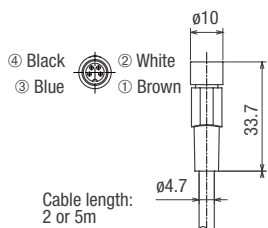
Straight (SA9Z-CM8K-4S□)
