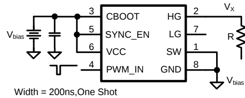
Figure 3. Test Circuit 2
