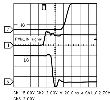
Figure 7. When Input Goes High
