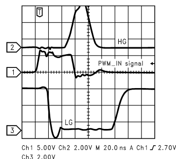
Figure 9. Minimum Positive Pulse
