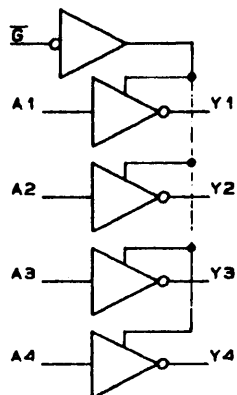
LOGIC DIAGRAM (1/2 CIRCUIT)
