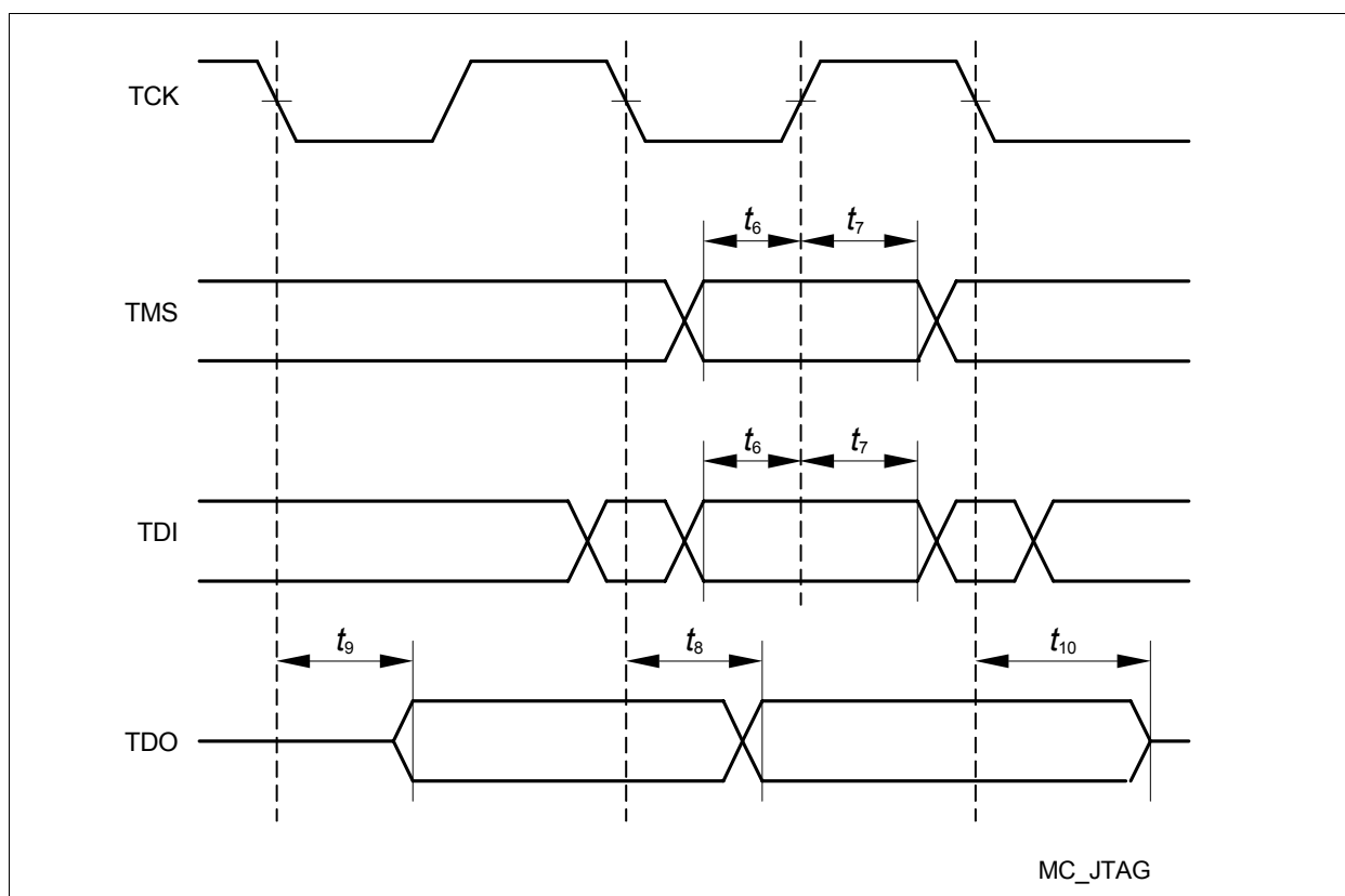
Figure 27 JTAG Timing
