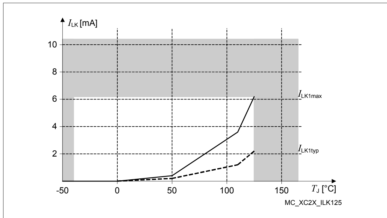
Figure 14 Leakage Supply Current as a Function of Temperature
