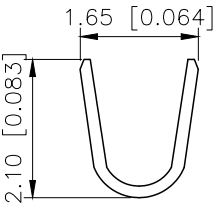
SECTION:A-A SCALE:1:1
