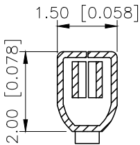
SECTION:C-C SCALE:1:1
