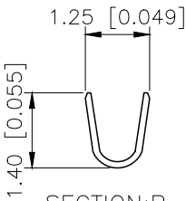
SECTION:B-B SCALE:1:1
